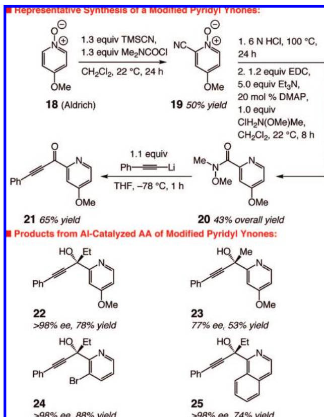
Scheme 2. Synthesis and Al-Catalyzed AA of Substrates with a Modified Pyridine
